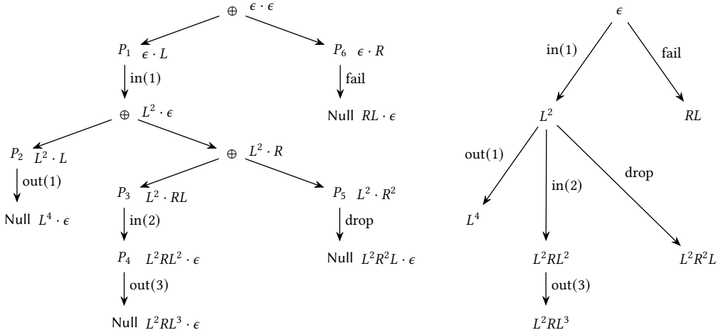
Fig. 5. Process P and the schedule \rho of Example 5.10 (left) and resulting canonical model (right). Each process (node in the left graph) is annotated with its position cpos = ppos \cdot x .
